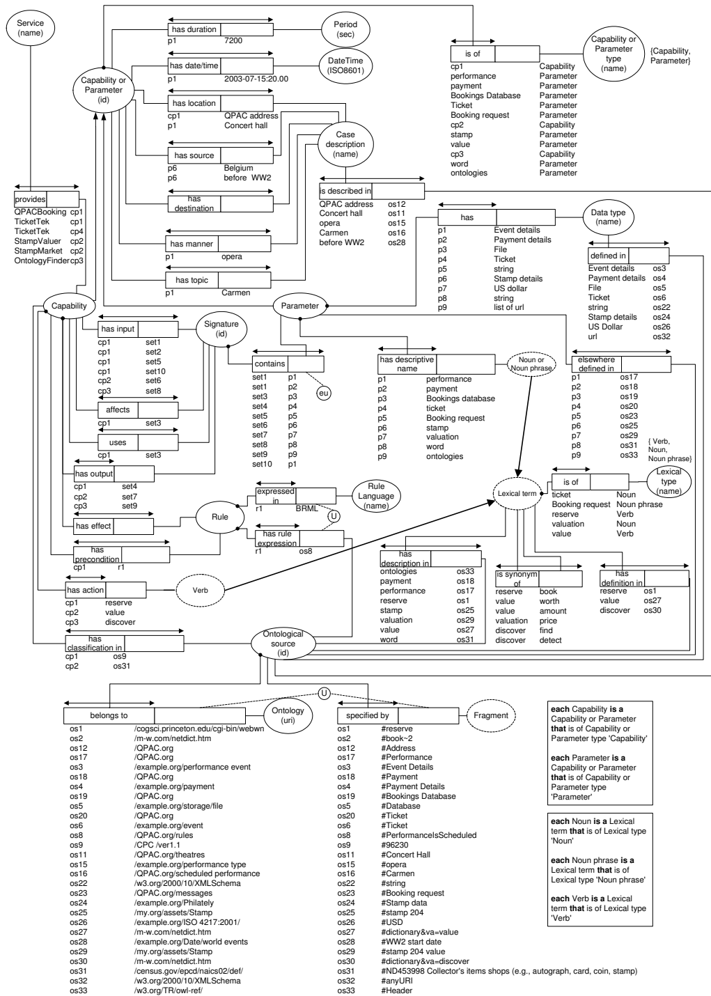
Fig. 1. A conceptual meta model of capability
